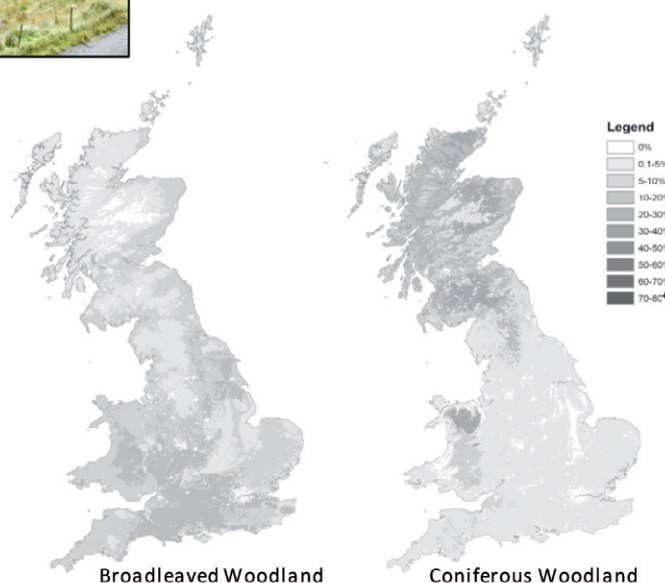
Figure 2. Countryside Survey 2007 % Estimates of Woodland Distribution in GB
